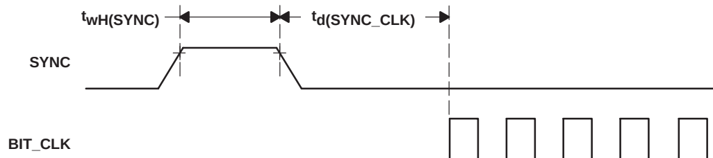
Figure 4-6. Warm Reset Timing
