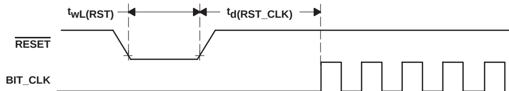
Figure 4-5. Cold Reset Timing
