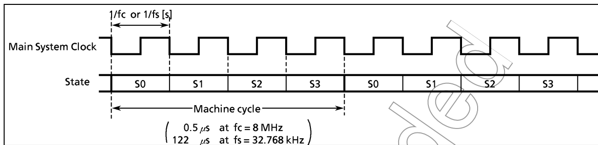
Figure 1-13. Machine Cycle
