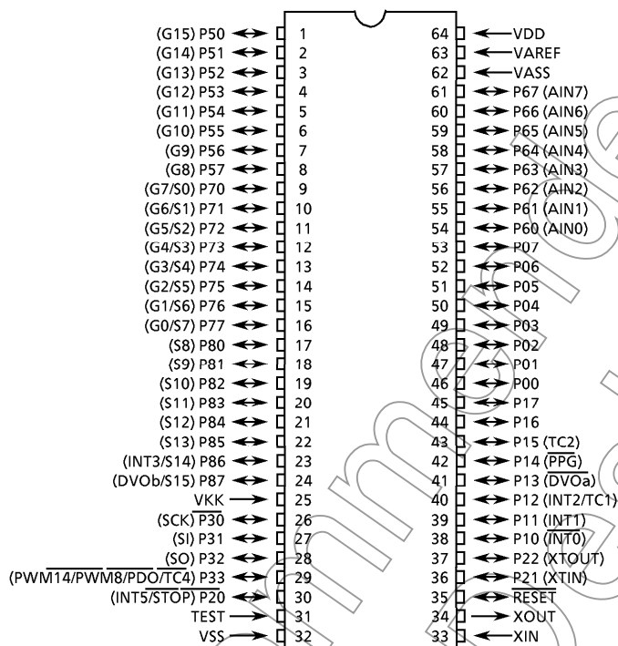
(1) P-SDIP64-750-1.78
