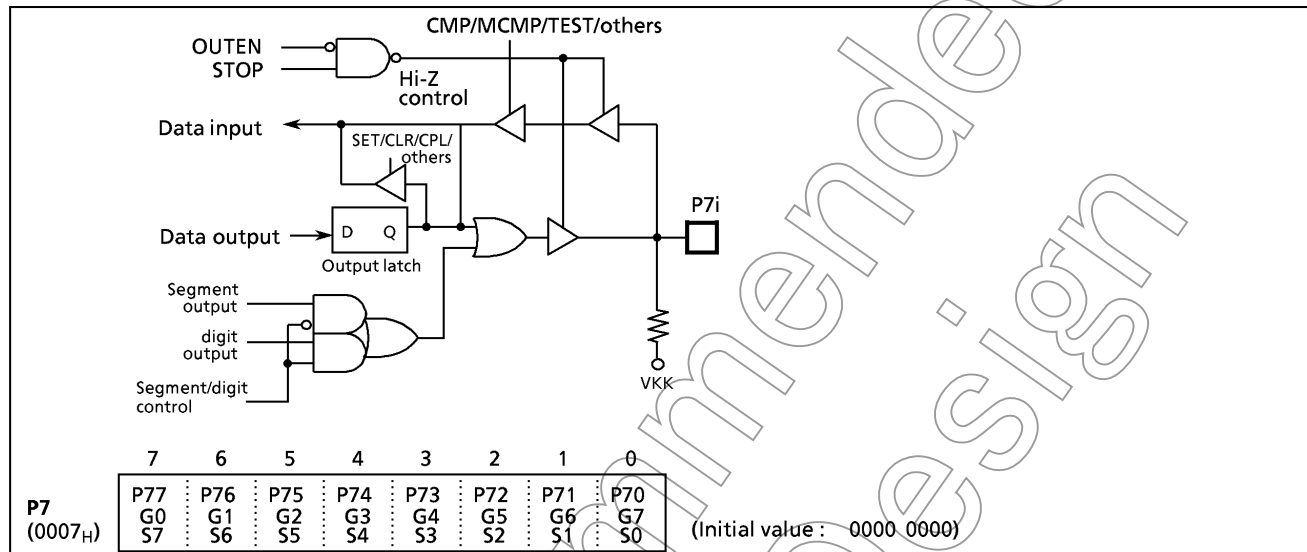
Figure 2-10. Port P7
