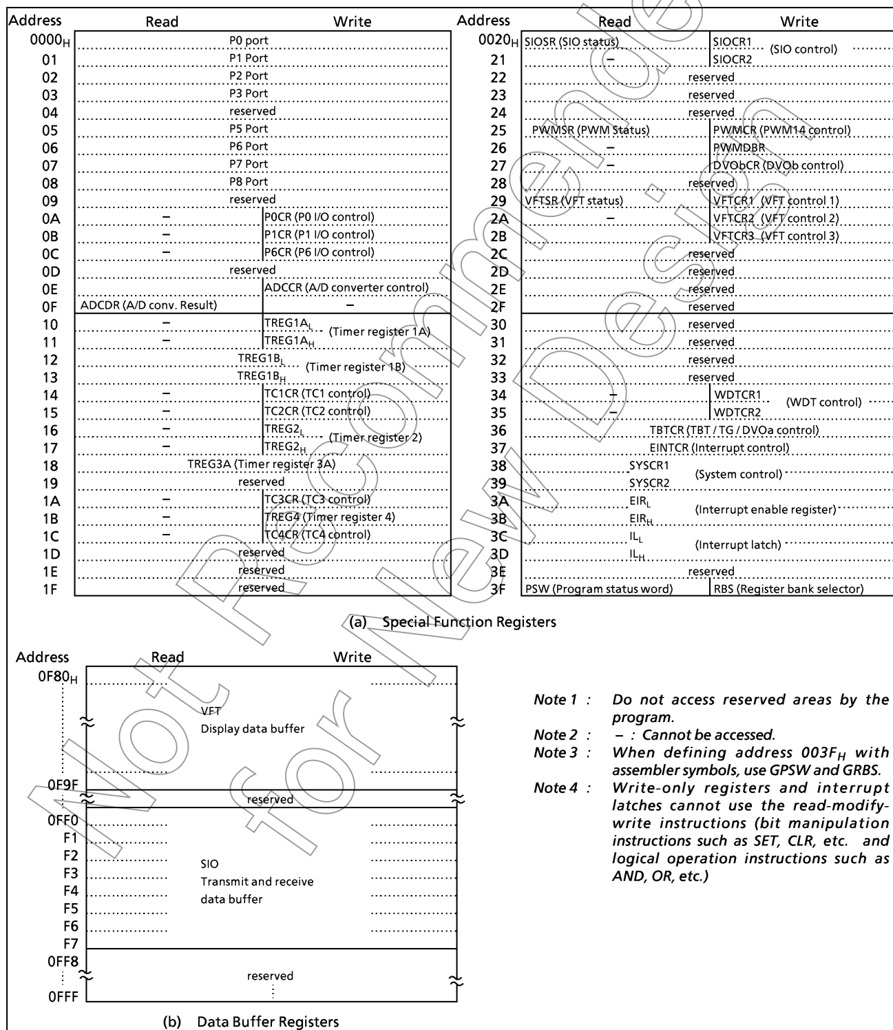
Figure 2-1. SFR & DBR
