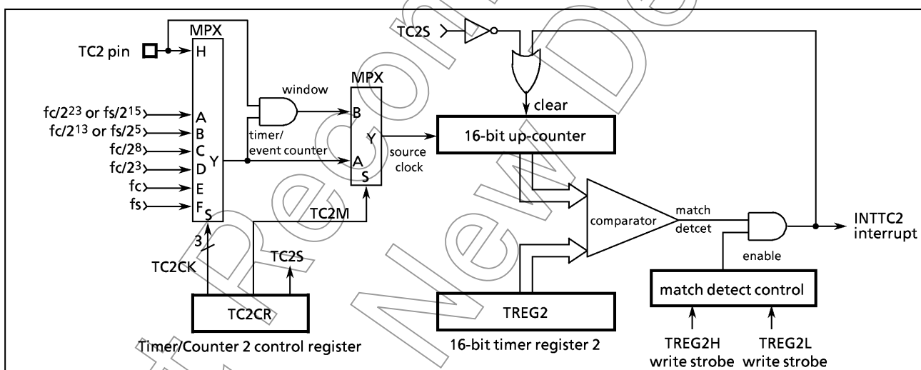
Figure 2-27. Timer/Counter 2 (TC2)
