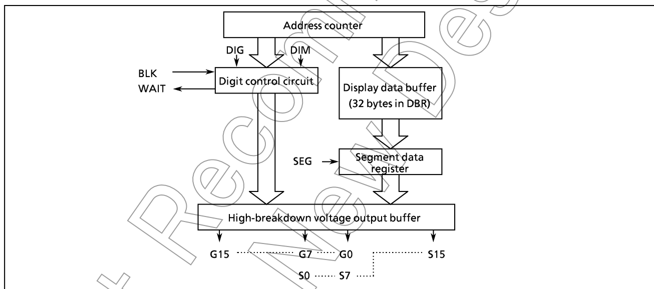
Figure 2-53. VFT
