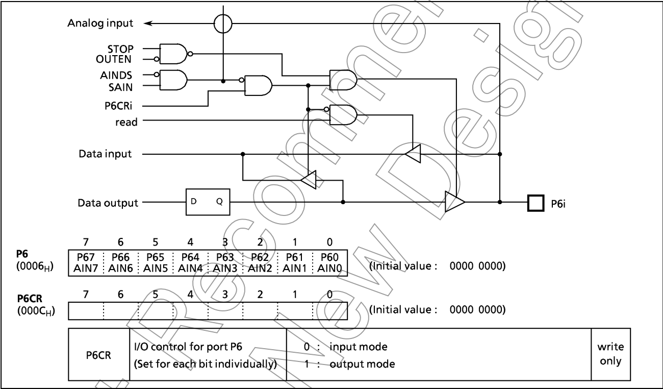
Figure 2-9. Port P6
