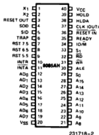
Figure 2. 8085AH Pin Configuration
