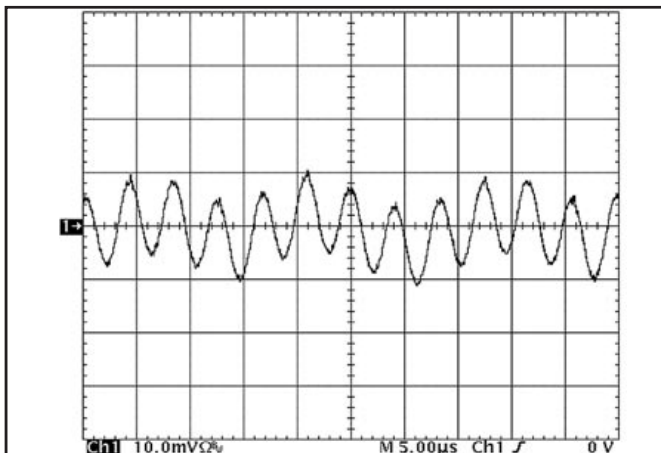
Figure 14: Input Terminal Ripple Current, i_c , at full rated output current and nominal input voltage with 10\ \mu H source impedance and 47\ \mu F electrolytic capacitor ( 100\ mA/div ). (See Figure 13)
