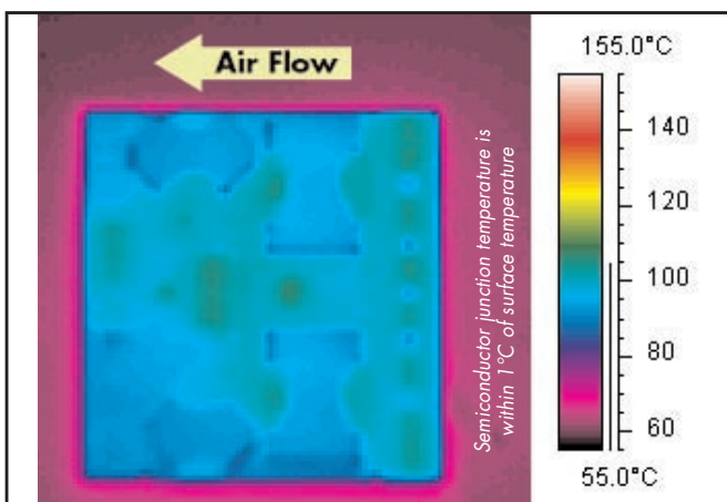
Figure 6: Thermal plot of converter at 40 amp load current with 55°C air flowing at the rate of 200 LFM. Air is flowing across the converter from output to input (nominal input voltage).
