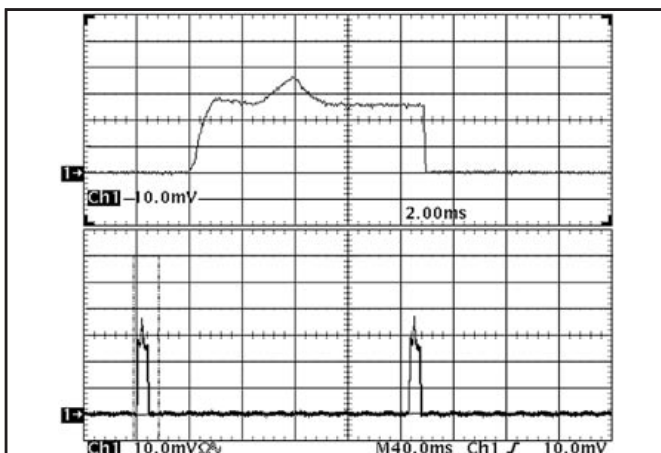
Figure 18: Load current ( 20A/div ) as a function of time when the converter attempts to turn on into a 1\ m\Omega short circuit. Top trace ( 2ms/div ) is an expansion of the on-time portion of the bottom trace.
