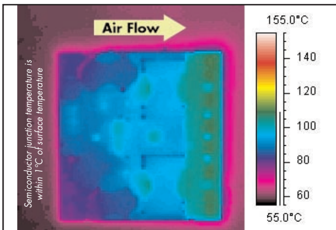
Figure 8: Thermal plot of converter at 40 amp load current with 55°C air flowing at the rate of 200 LFM. Air is flowing across the converter from input to output (nominal input voltage).
