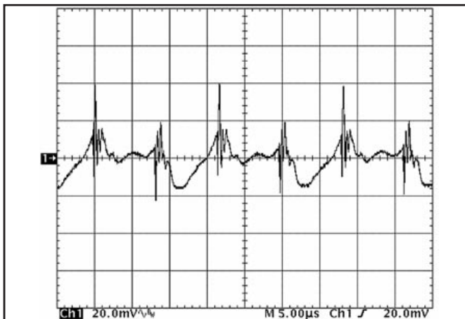
Figure 16: Output voltage ripple at nominal input voltage and rated load current ( 20\ mV/div ). Load capacitance: 1\ \mu F ceramic capacitor and 15\ \mu F tantalum capacitor. Bandwidth: 20\ MHz . (See Figure 13)
