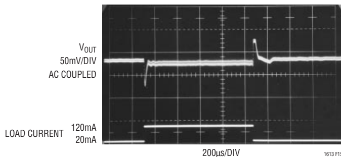
Figure 15. 5V Output SEPIC with 10µF Ceramic Output Capacitor, 330pF C_{PL} and 10k in Series with FB Pin
