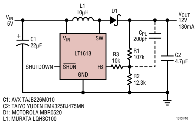
Figure 10. 5V to 12V Boost Converter with 4.7µF Ceramic Output Capacitor, C_{PL} Added to Increase Phase Margin
