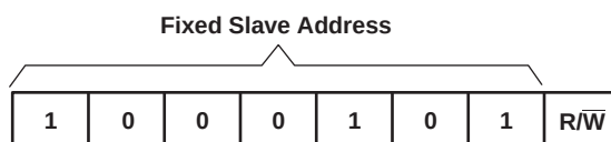
Figure 17. TCA6507 Address
