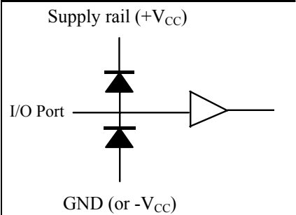
Steering Diode Application
