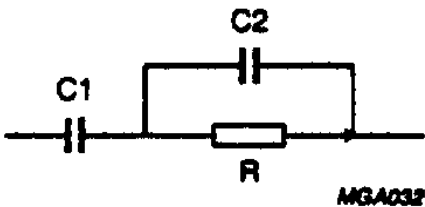
Fig.8 Loop filter.
