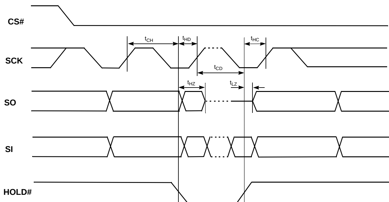
Figure 27. HOLD# Timing
