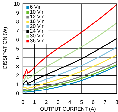
Figure 22. Dissipation 1.8-V Output at 85°C
