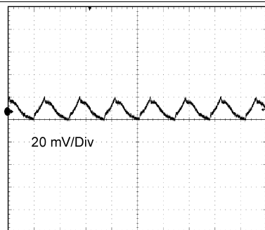
Figure 33. Output Ripple
