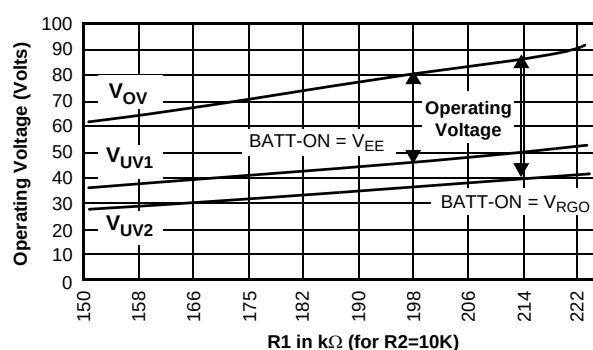
Figure 8. Operating voltage vs. resistor ratio
