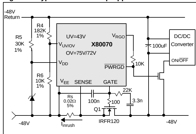
Figure 6. Typical -48V Hotswap Application circuit
