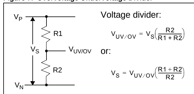
Figure 7. Overvoltage Undervoltage Divider
