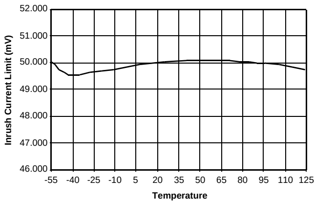
Overcurrent Threshold vs. Temperature
