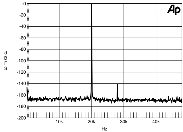
Figure 34. Wideband FFT Plot (16k Points) 0 dBFS 20 kHz Tone, 48 kHz:96 kHz
