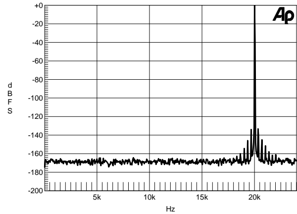
Figure 36. Wideband FFT Plot (16k Points) 0 dBFS 20 kHz Tone, 96 kHz:48 kHz
