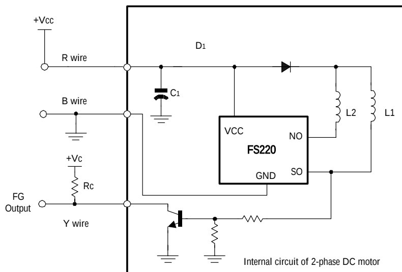
Fig 5 Application Circuit
