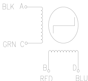
4 Leads
