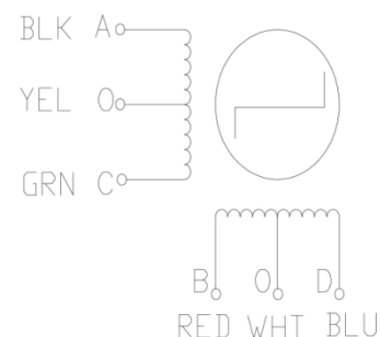
6 Leads
