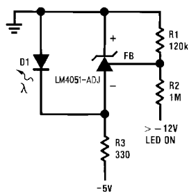
Figure 24. Fast Positive Clamp 2.4V + V_{D1}
