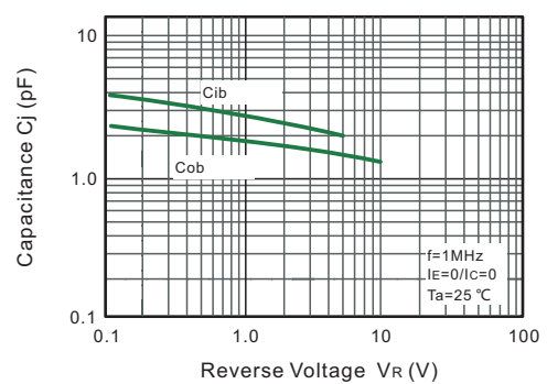
Fig.8 Cob/Cib-VCS/VEB
