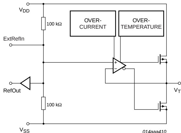
Fig 7. Block diagram
