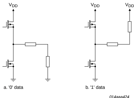
Fig 6. V_{TT} loading conditions
