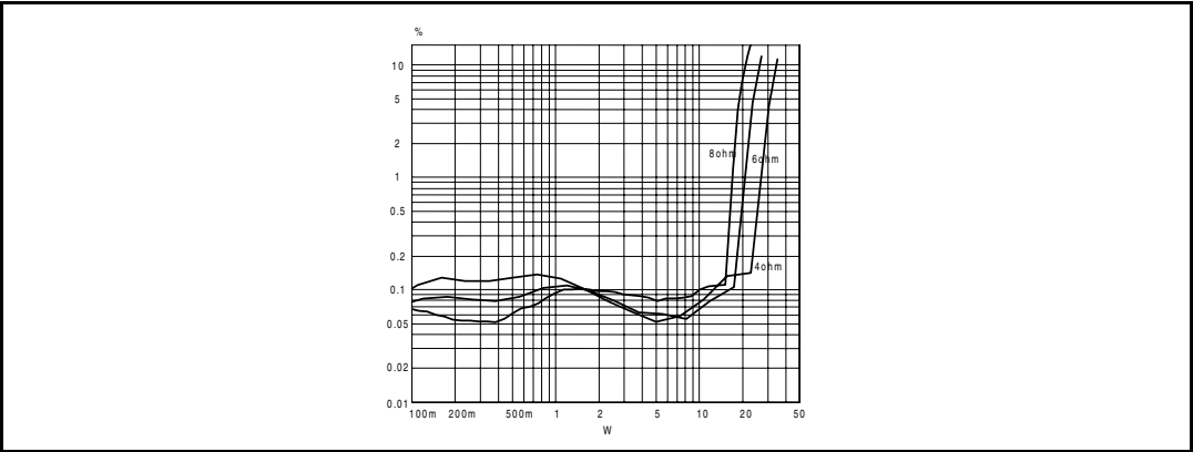
Figure 23. THD vs. PWR BTL, 1 kHz
