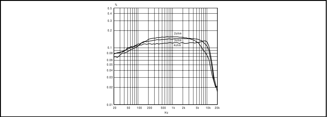
Figure 37. THD against freq SE 1 W
