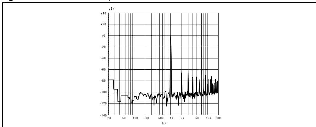
Figure 28. FFT 0 dbfs 1 kHz, 1 kHz 4 \Omega
