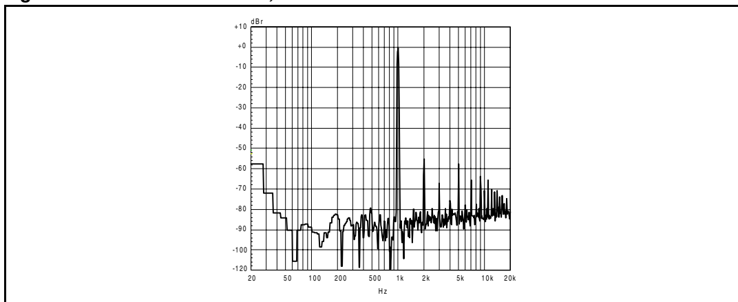
Figure 40. FFT 0 dB 1 kHz SE, 3 \Omega
