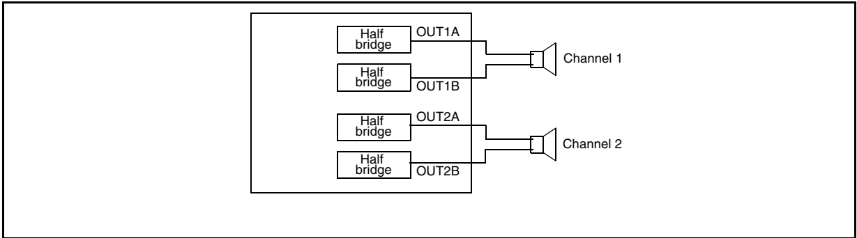
Figure 4. 2-channel (full-bridge) power, OCFG(1...0) = 00
