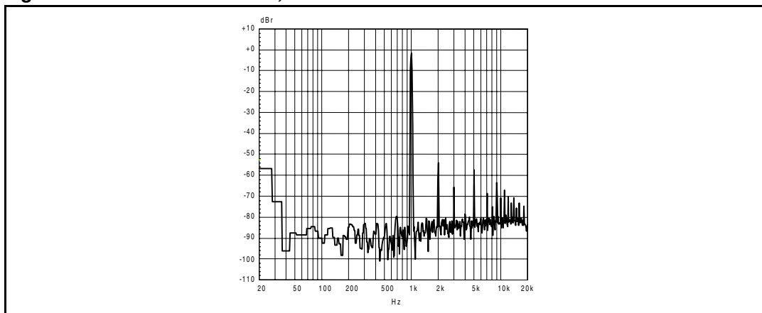
Figure 41. FFT 0 dB 1 kHz SE, 4 \Omega
