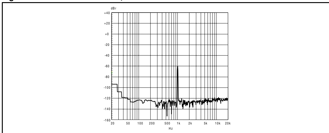
Figure 30. FFT -60 dbfs 1 kHz, 6 \Omega
