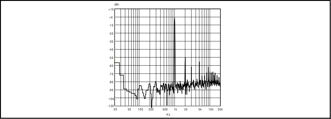
Figure 39. FFT 0 dB 1 kHz SE, 2 \Omega
