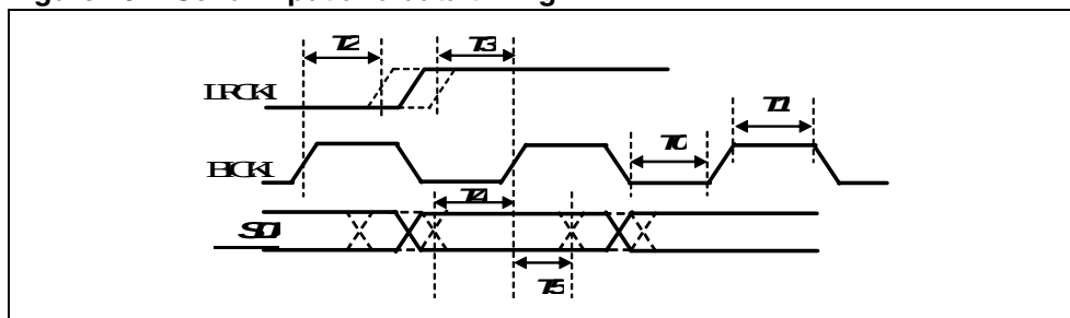
Figure 49. Serial input and data timing
