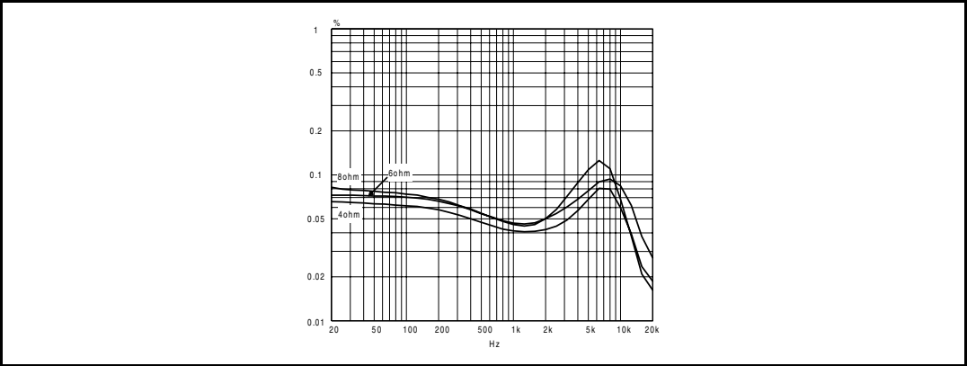
Figure 25. THD vs. freq. BTL 16 W output
