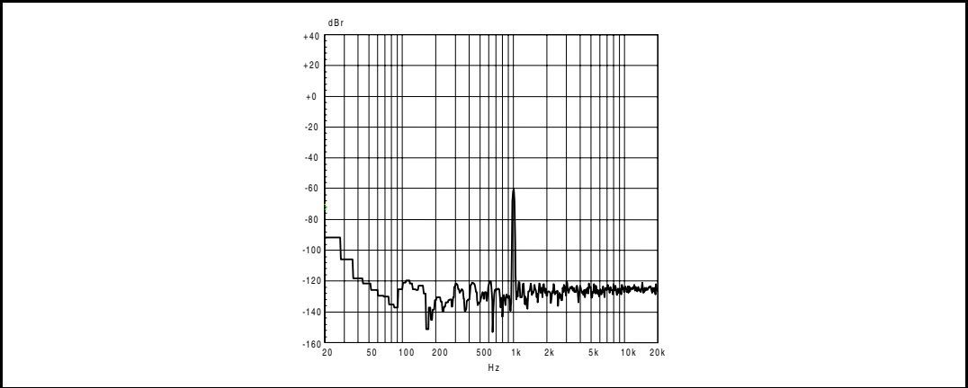
Figure 31. FFT -60 dbfs 1 kHz, 4 Ω
