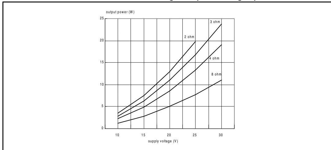
Figure 16. Half bridge binary mode output power vs. supply voltage (THD+N=1%). Curves taken at 1 kHz and using a 330 \mu F blocking capacitor
