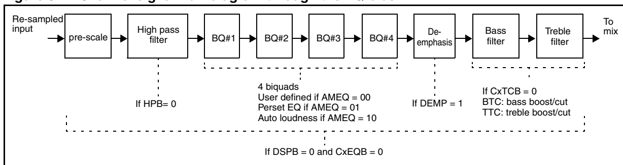
Figure 3. Channel signal flow diagram through the EQ block
