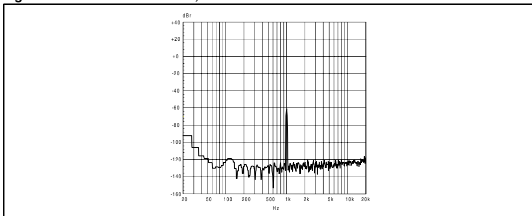
Figure 29. FFT -60 dbfs 1 kHz, 8 \Omega
