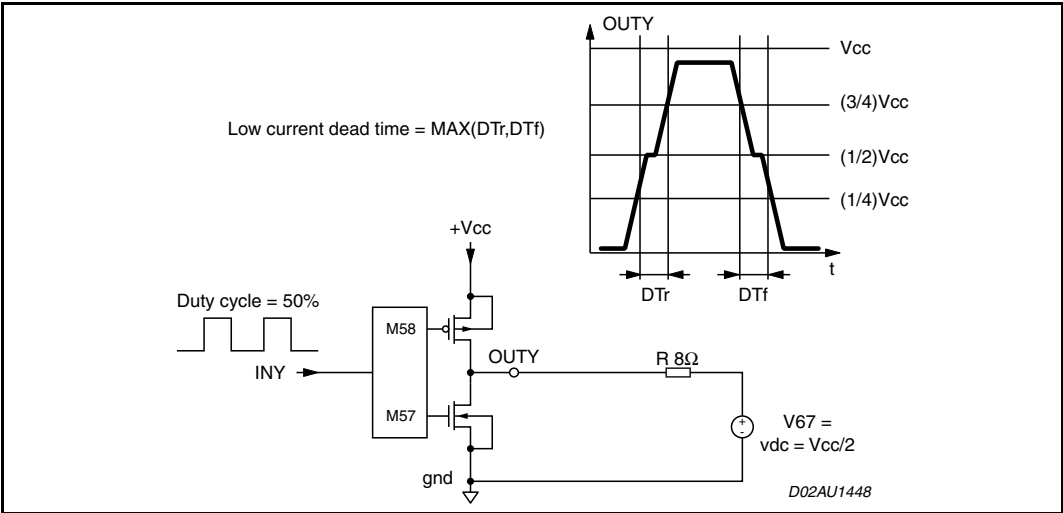
Figure 11. Test circuit
