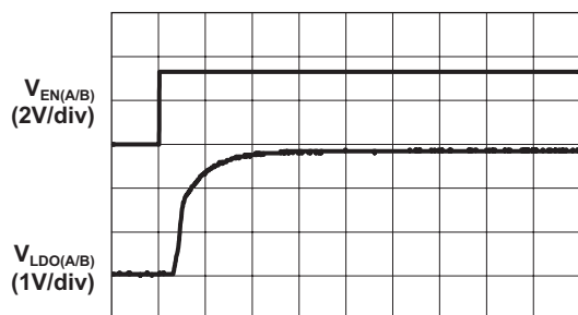
LDOA/LDOB Turn On ( V_{IN} = 3.6V ; V_{LDO(A/B)} = 2.8V ; DC Coupled)
