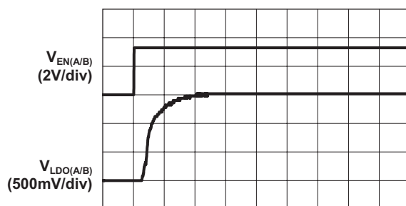
LDOA/LDOB Turn On ( V_{IN} = 3.6V ; V_{LDO(A/B)} = 1.5V ; DC Coupled)
