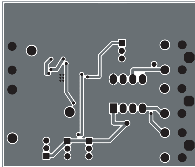
Figure 6: AAT2847 Evaluation Board Solder Side Layout.
