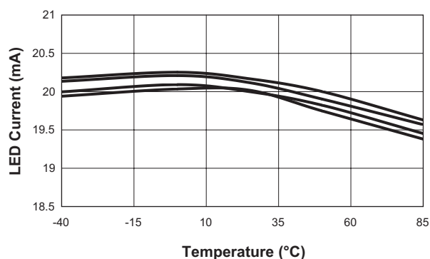
Backlight Current Matching vs. Temperature (I_{OUT} = 20\text{mA/Channel}; V_{IN} = 4.2\text{V})
