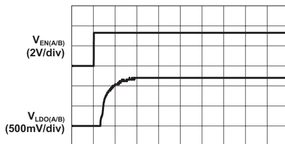
LDOA/LDOB Turn On ( V_{IN} = 3.6V ; V_{LDO(A/B)} = 1.2V ; DC Coupled)
