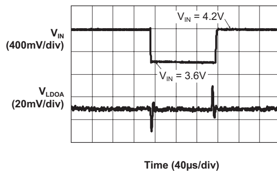
LDOA Line Transient Response (10mA Load)
