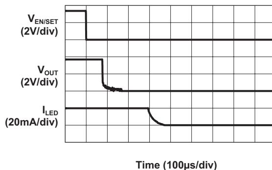
Turn Off from 1.5X Mode Backlight (20mA/Channel; Address 0, Data 1; V_{IN} = 3.6V )
