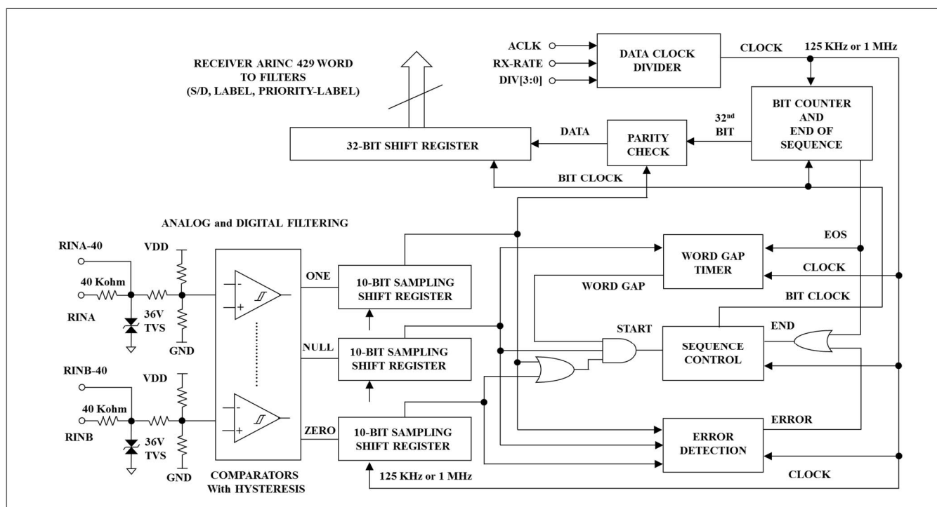
Figure 8 Receiver function diagram
