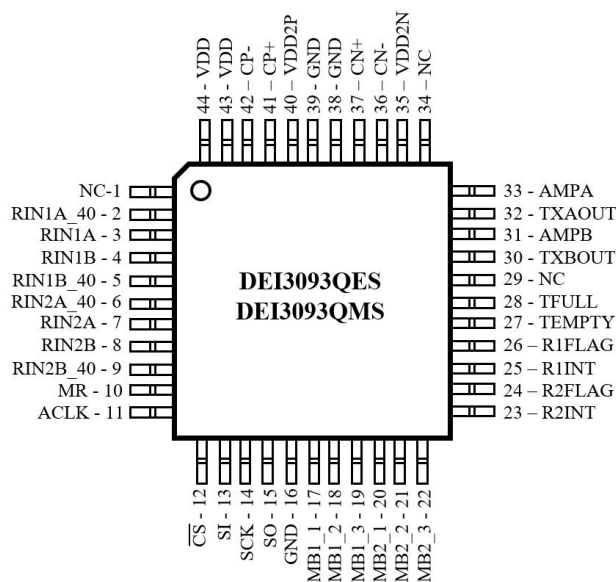
44L PQFP (top view)
