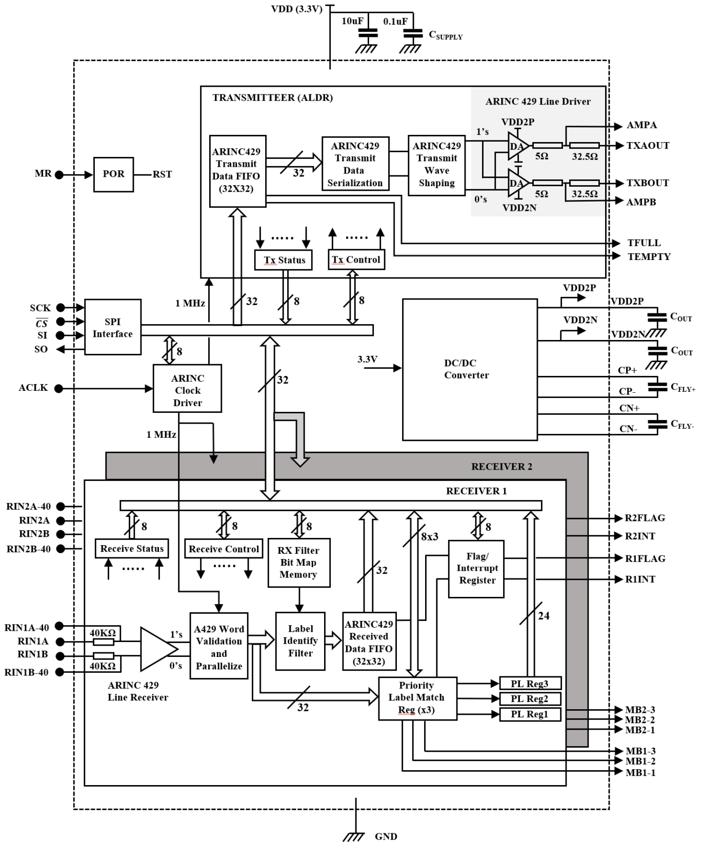
Figure 1 Function Diagram
