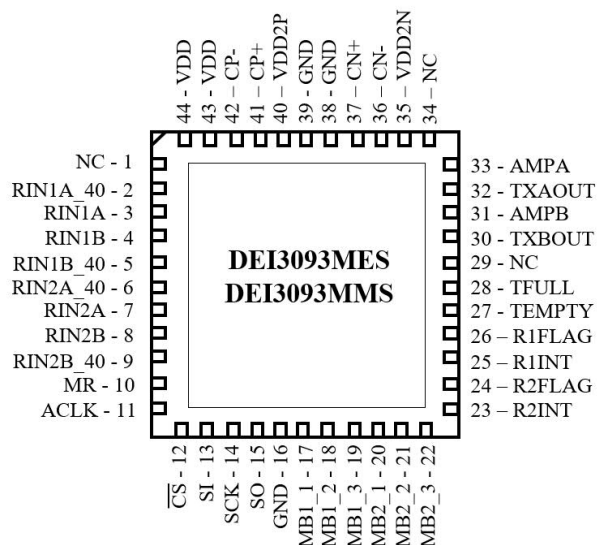
44L QFN (top view)
