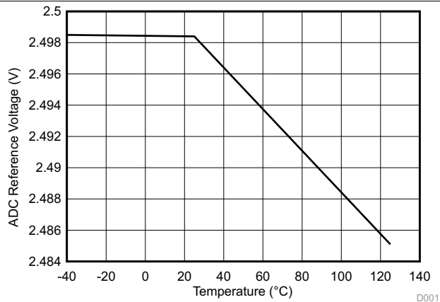
Figure 3. ADC Reference Voltage vs Temperature
