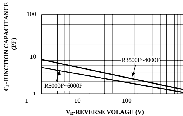
FIG. 6-TYPICAL JUNCTION CAPACITANCE
