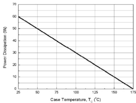
Fig. 5 Power Derating
