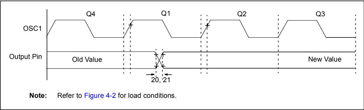
FIGURE 4-4: OUTPUT WAVEFORM
