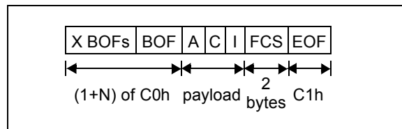
FIGURE 2-8: IRLAP FRAME
