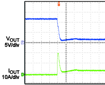
0.33Ω Load Connected to Enabled Device
