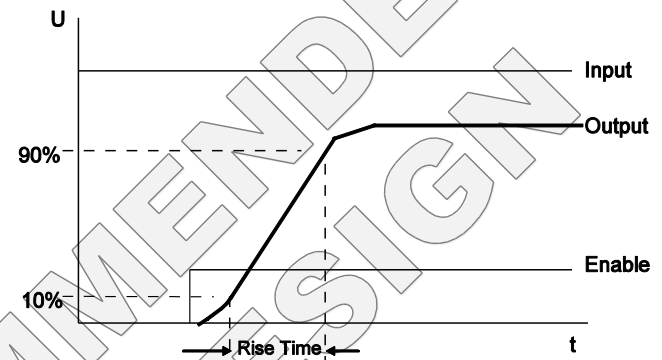
Figure 2—Rise Time
