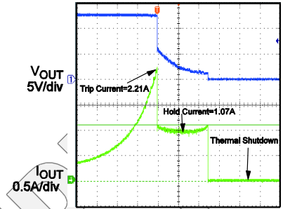
Current Limit R_{LIMIT} = 100\Omega
