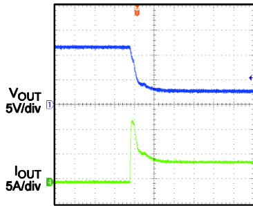
0.66Ω Load Connected to Enabled Device
