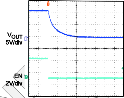
Turn Off Delay and Fall Time with 1 \mu F Load
