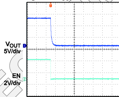
Turn Off Delay and Fall Time with 10 \mu F Load
