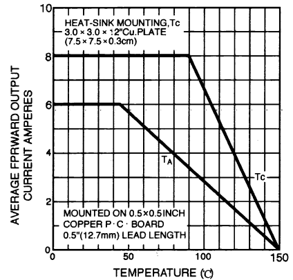
FIG. 2 – TYPICAL FORWARD OUTPUT DERATING CURVE
