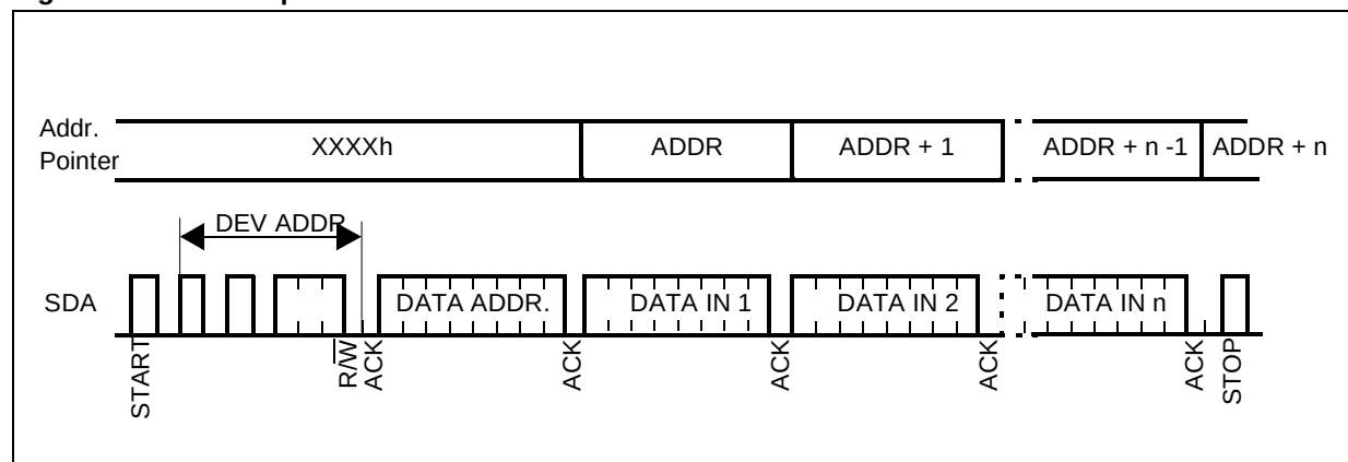
Figure 65. Write sequence
