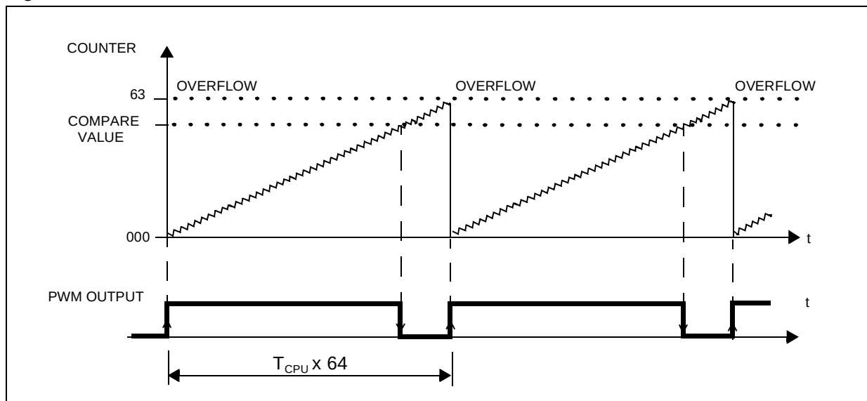
Figure 69. PWM Generation
