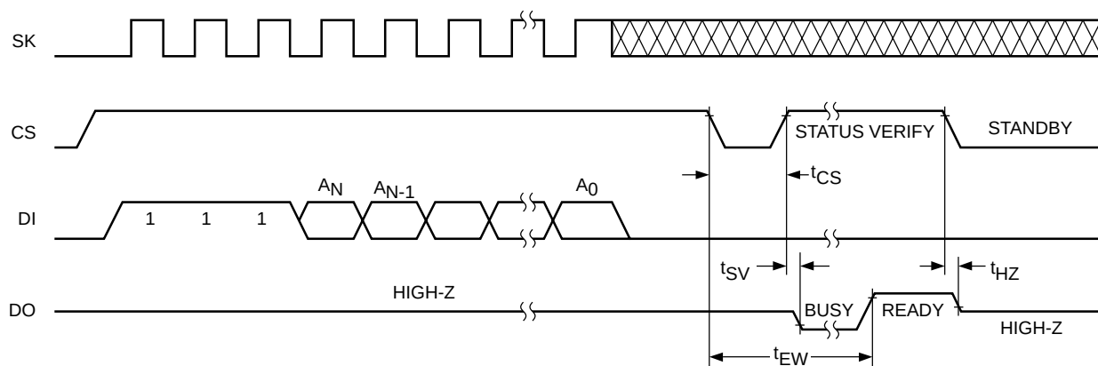
Figure 4. Erase Instruction Timing
