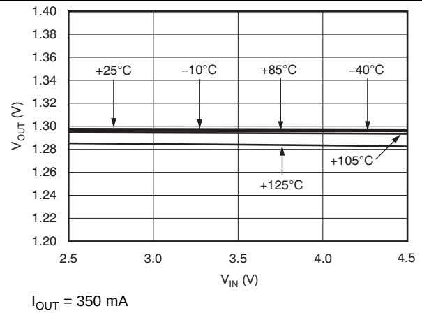
Figure 2. V_{\text{IN}} Line Regulation (TPS72013YZU)
