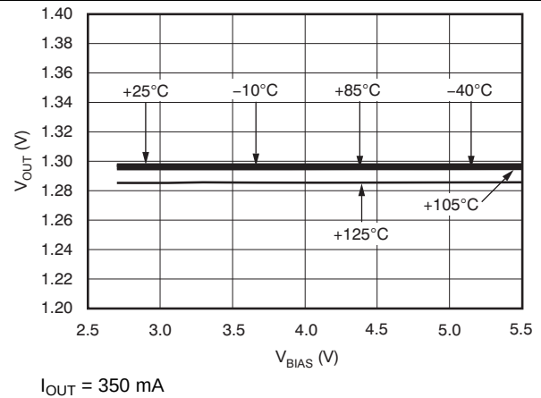
Figure 4. V_{\text{BIAS}} Line Regulation (TPS72013YZU)
