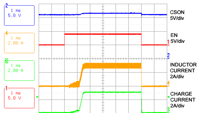
FIGURE 10. CHARGE ENABLE AND SHUTDOWN
