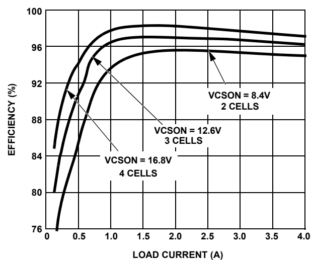
FIGURE 7. SYSTEM EFFICIENCY vs CHARGE CURRENT
