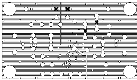
Figure 45. AD8436-EVALZ Power Plane
