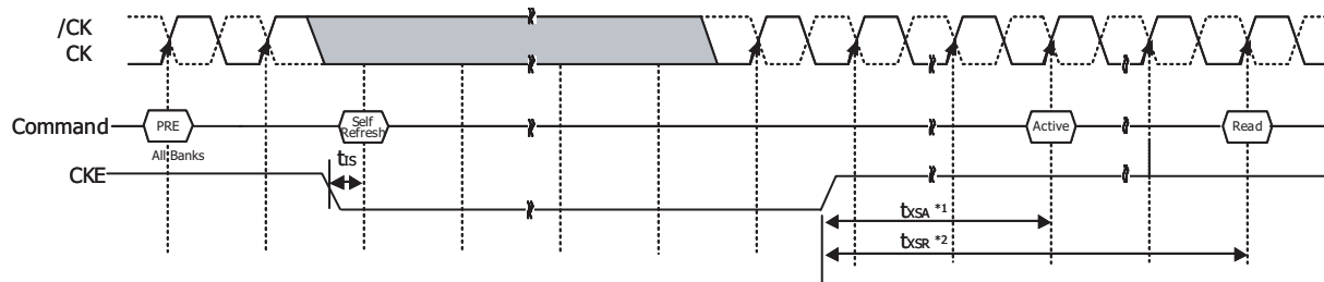
Figure 21: Self Refresh
