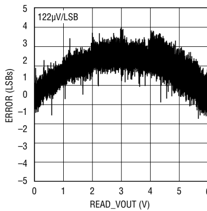
ADC READ_VOUT-INL
