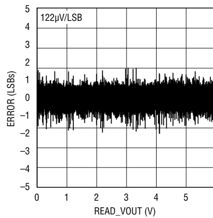
ADC READ_VOUT-DNL
