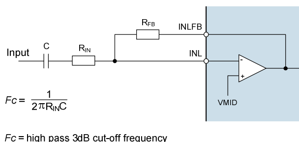
Figure 14 Input Signal Path External Components
