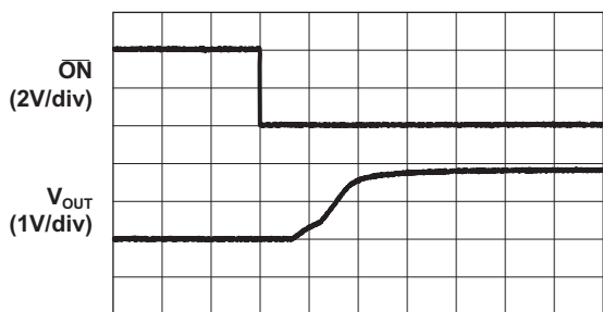
Power-Up with 1mA Load
