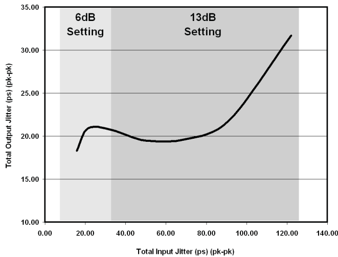
A. DisplayPort output jitter measured at the surface mount pins connected to the main link output channels on the SN75DP130 characterization test board; input jitter generated from test board with variable input trace lengths using 4 mil traces of lengths 2 inches to 22 inches generating the typical input jitter as represented in Table 1.
