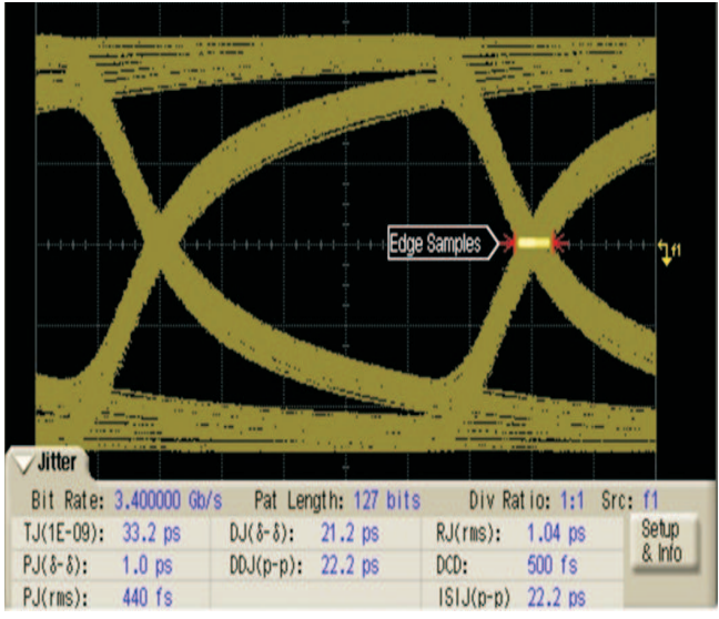
Figure 17. Main Link Input with 10 inch Trace; TMD5 Sink
