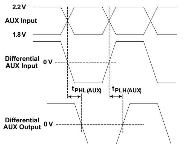
Figure 11. AUX Delay Measurement
