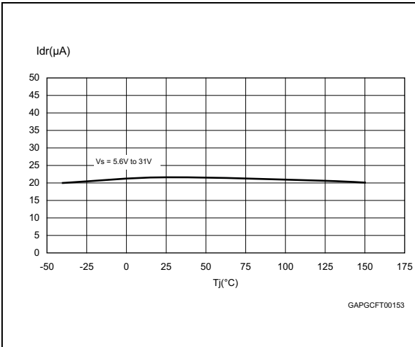
Figure 19. I_{dr} vs. T_j
