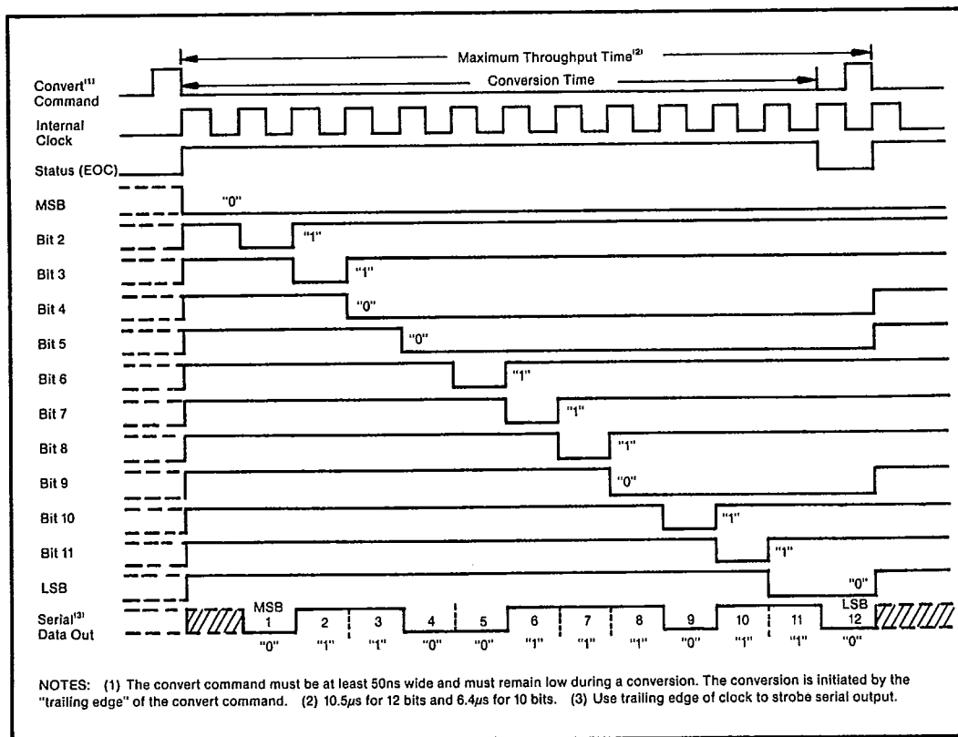
FIGURE 2. Timing Diagram.
