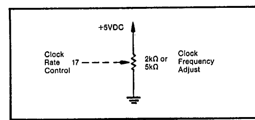
FIGURE 8. 12-Bit Clock Rate Control Optional Fine Adjust.
