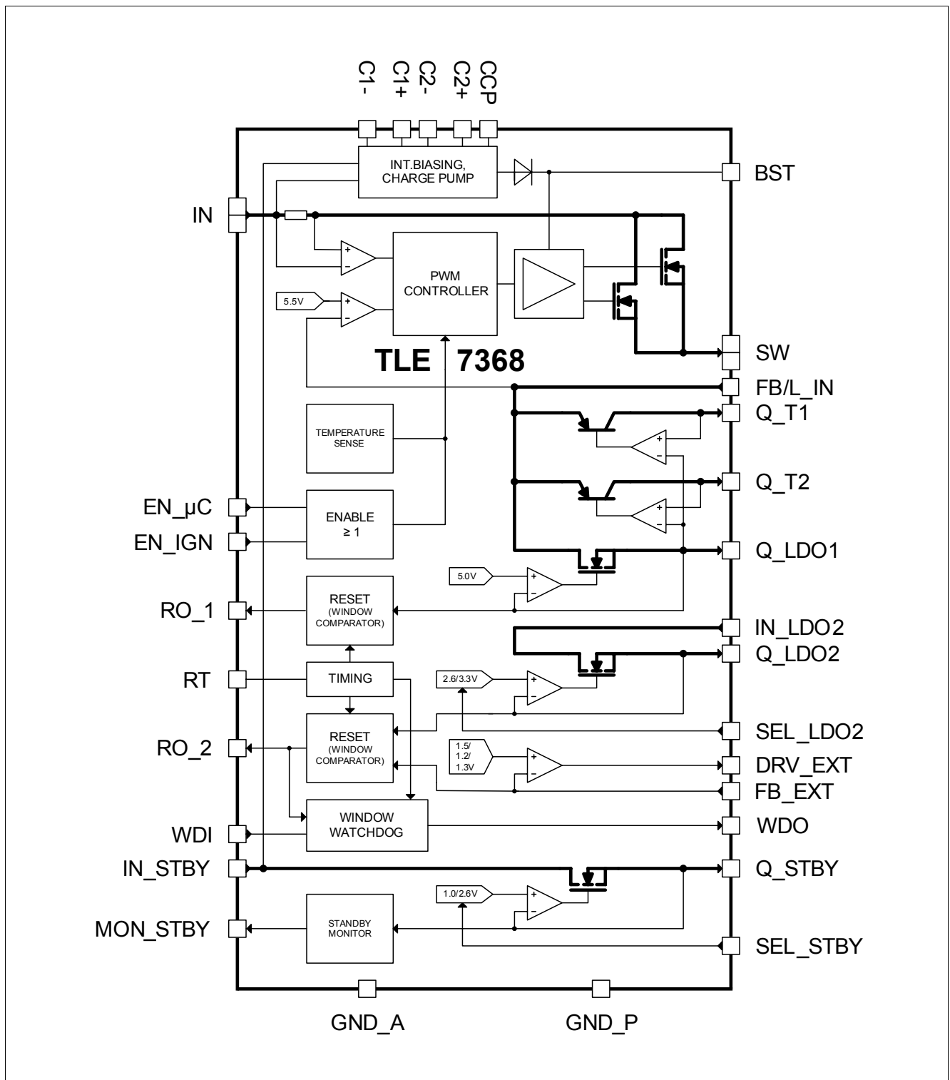
Figure 1 Block Diagram
