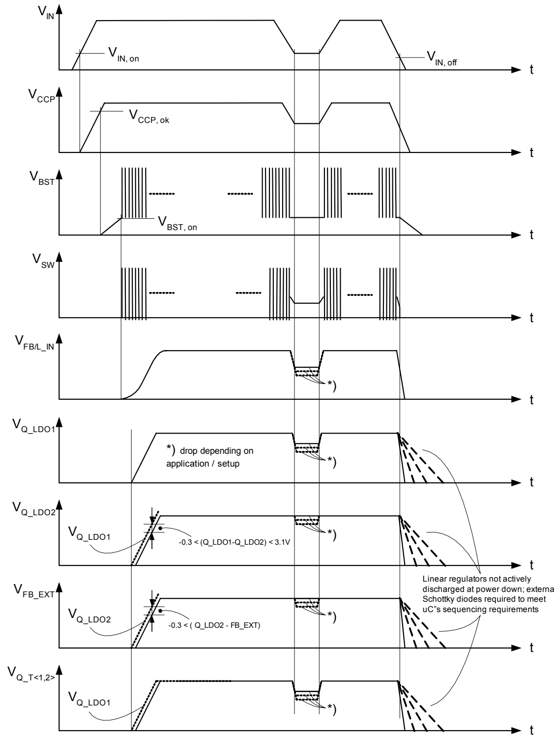
Figure 4 Power Sequencing of the TLE7368
