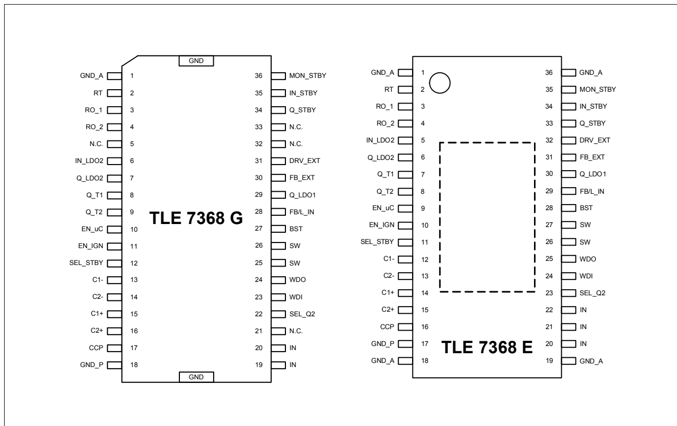
Figure 2 Pin Configuration
