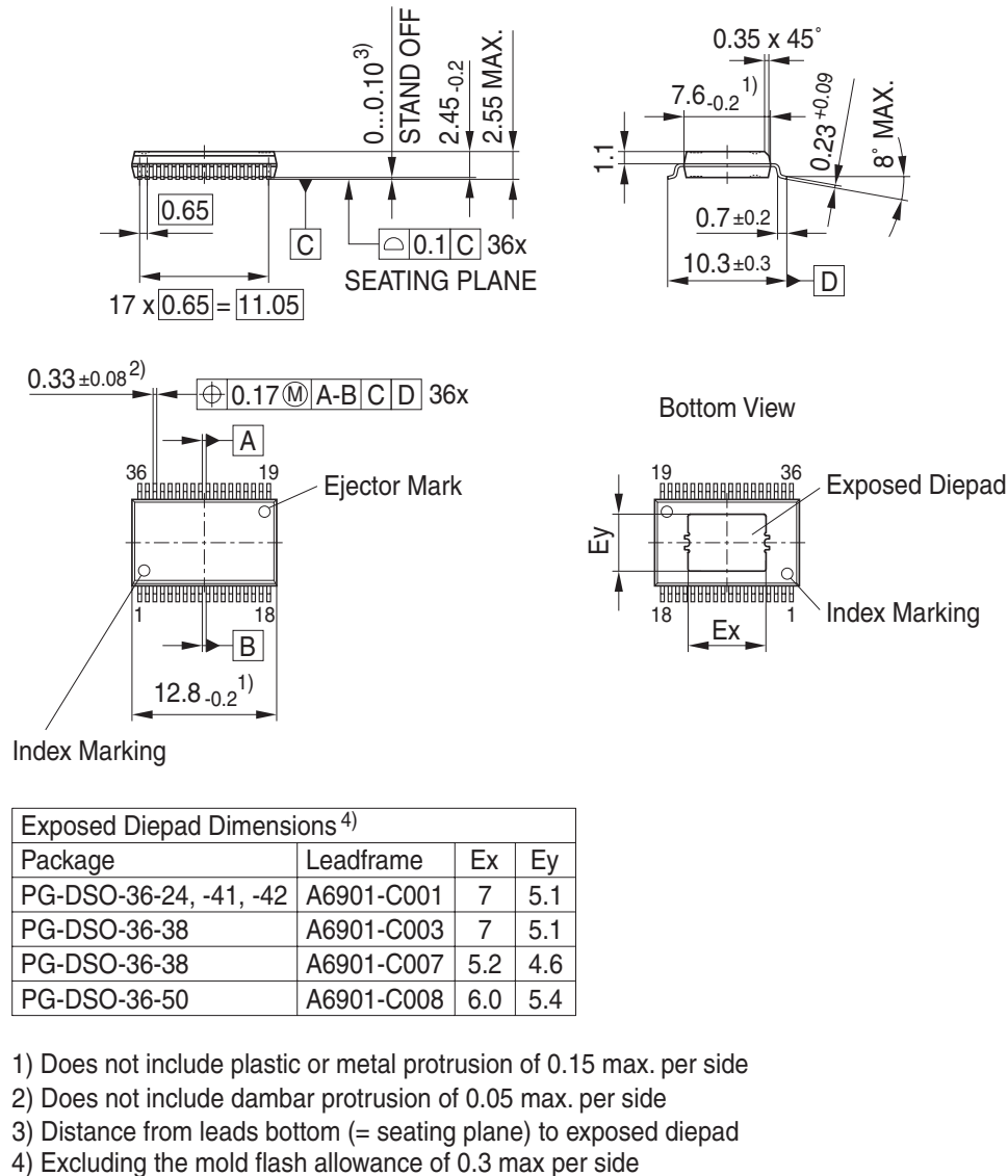
Figure 12 PG-DSO-36 (Plastic Green - Dual Small Outline Package)
