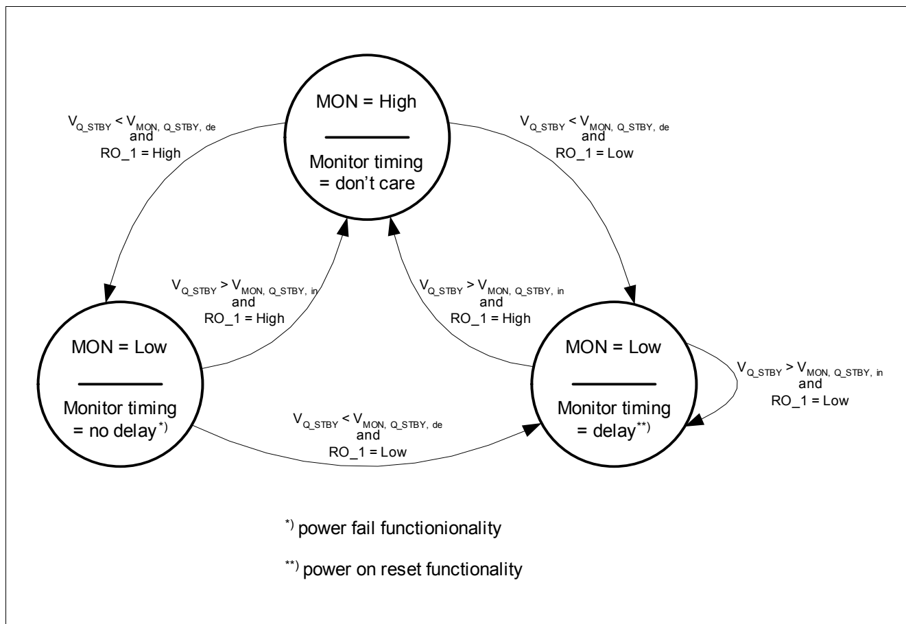
Figure 6 Stand by Monitor State Diagram
