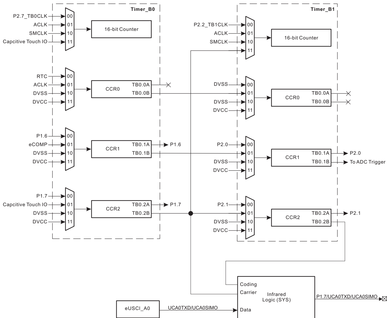
Figure 6-2. Timer_B Connections
