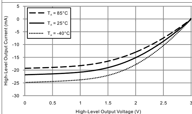
Figure 5-8. Typical High-Level Output Current vs High-Level Output Voltage (DVCC = 3 V)
