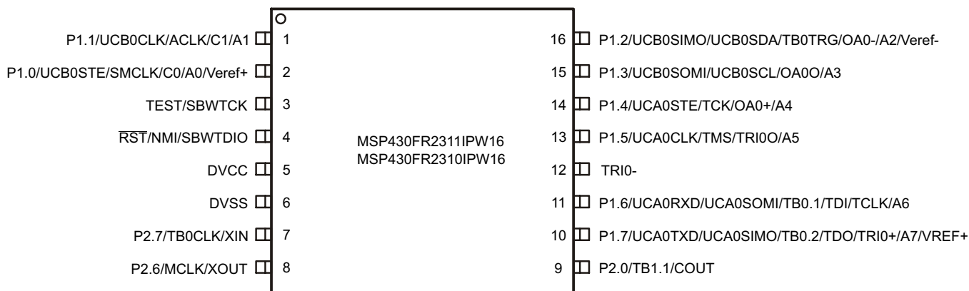
Figure 4-3. 16-Pin PW (TSSOP) (Top View)
