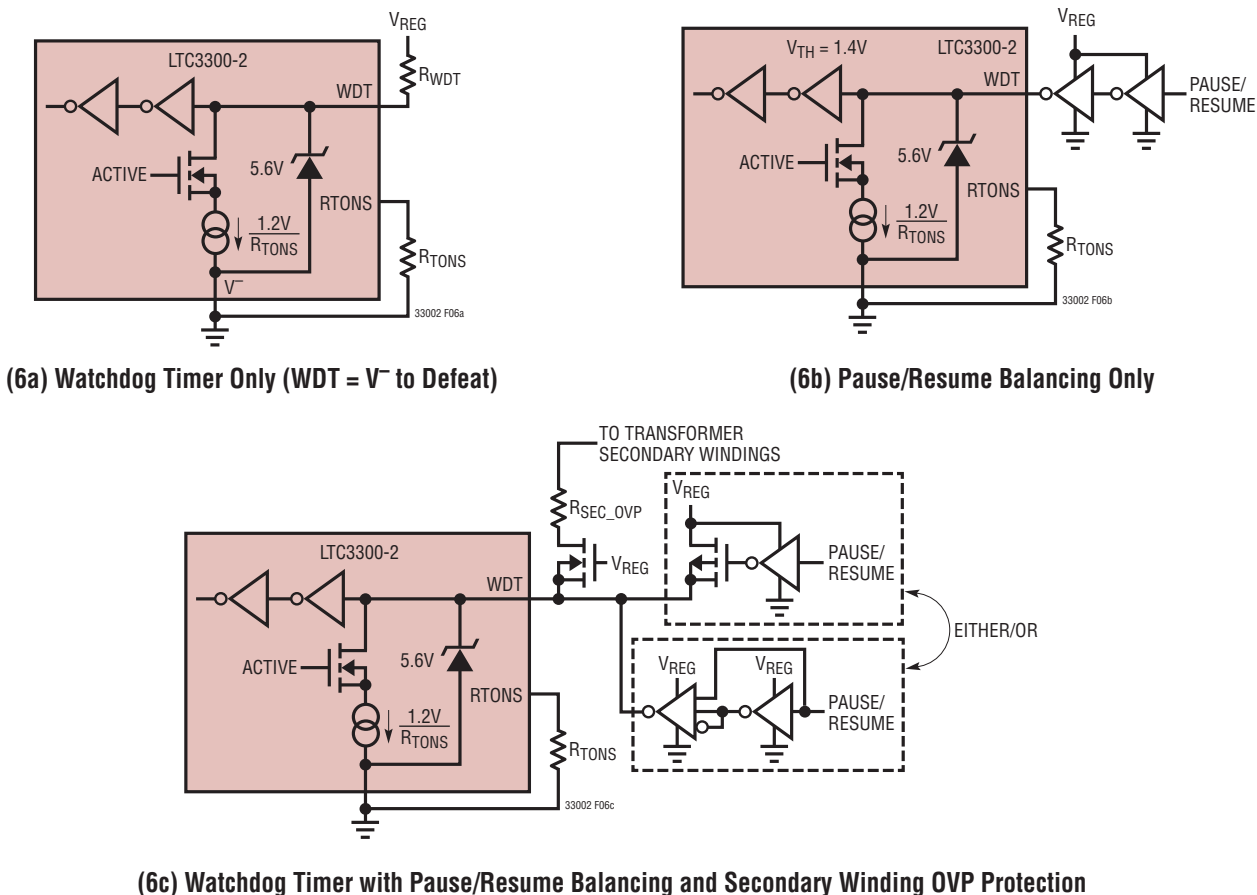
Figure 6. WDT Pin Connection Options
