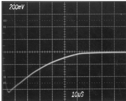
Transient Response for 0–5A Load Step
