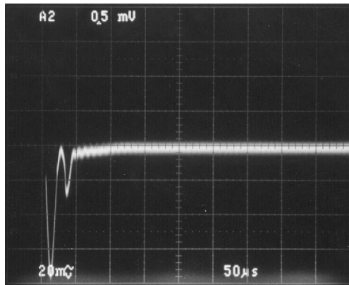
Transient Response with Output Capacitor Halved
