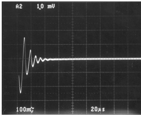
Transient Response with Only 4.7 \mu\text{F} Output Cap
