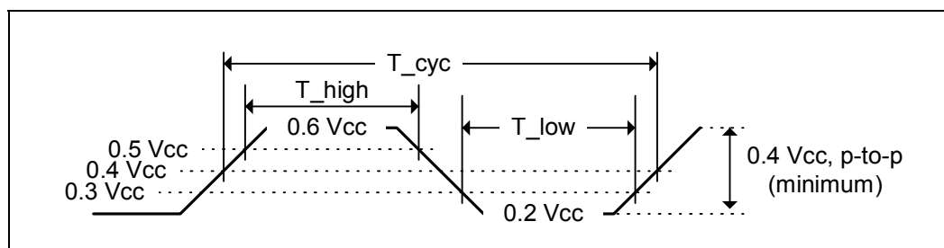
Figure 4-8. PCI-X 3.3V Clock Waveform
