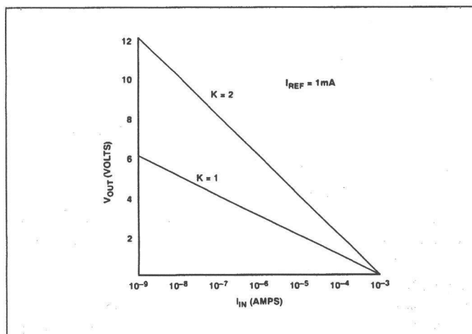
FIGURE 2a: Inverting Log Amp with Current Input
