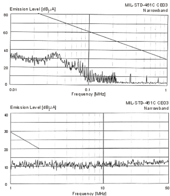
Figure 19 – DVFL2800S with EMI Filter
