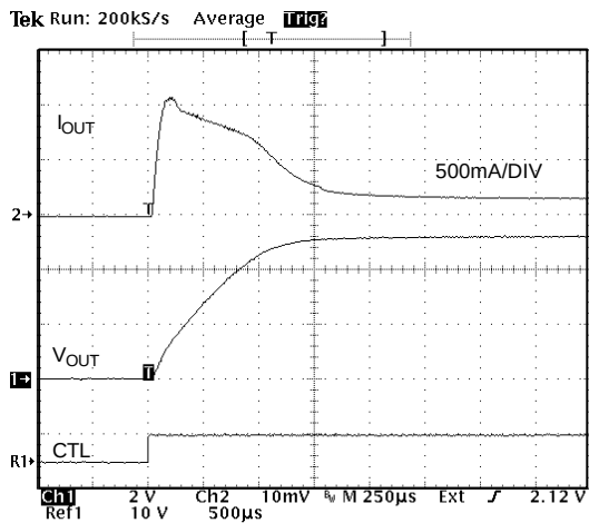
Turn On Characteristic ( 35\Omega , 100\mu\text{F} Loading)
