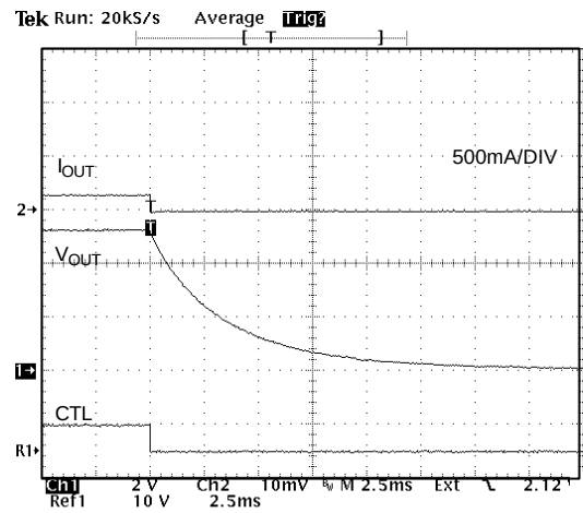
Turn Off Falling Time ( 35\Omega , 100\mu\text{F} Loading)
