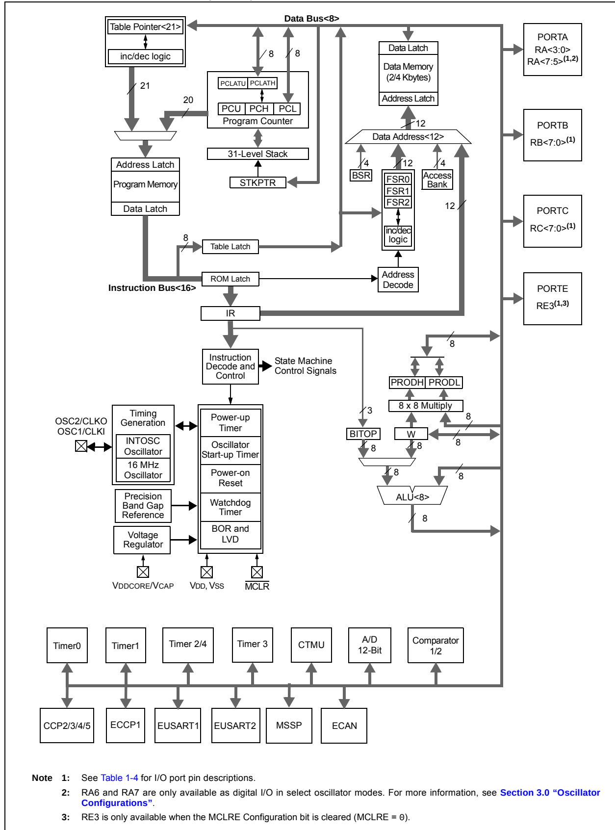
FIGURE 1-1: PIC18F2XK80 (28-PIN) BLOCK DIAGRAM
