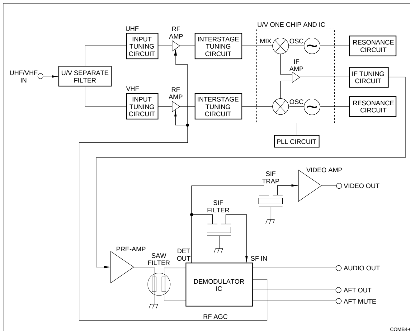
Figure 1. VTBT5UF201 Block Diagram
