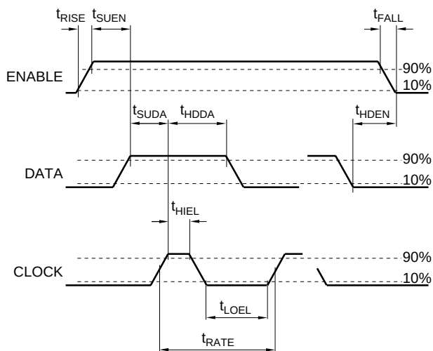
Figure 5. PLL AC Characteristics
