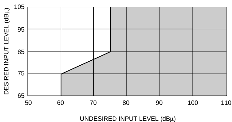
Figure 4. Cross Modulation Between Adjacent Channels
