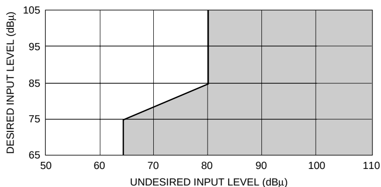
Figure 3. Cross Modulation Between Next and Adjacent Channels
