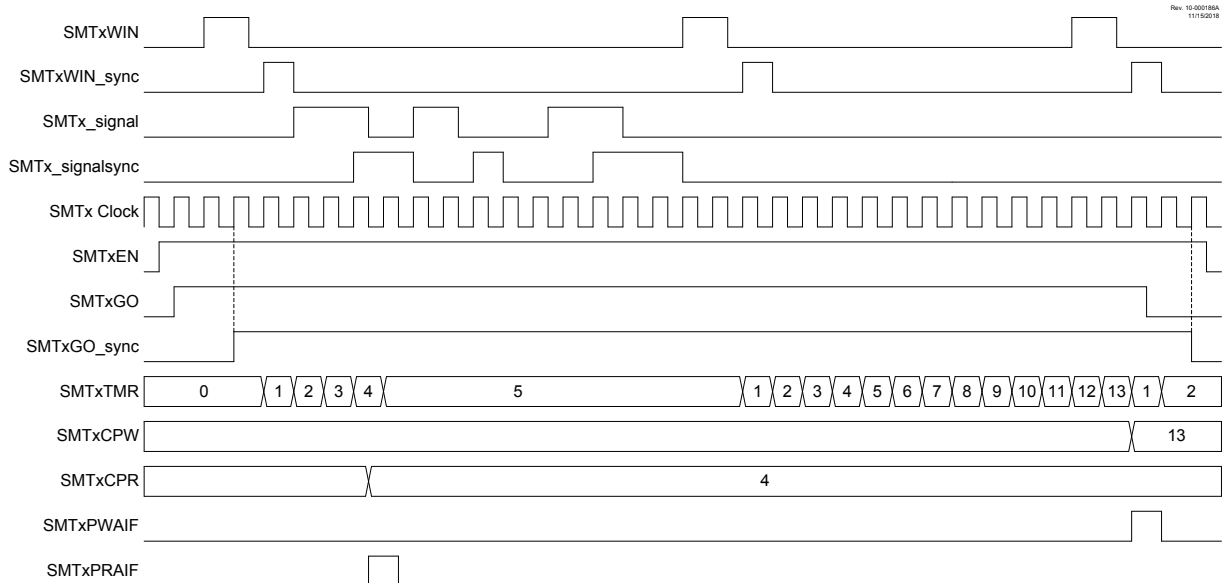
Figure 27-15. Time-of-Flight Mode, Single Acquisition Timing Diagram
