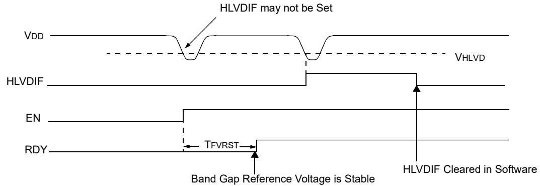
Figure 37-2. Low-Voltage Detect Operation (INTL = 1)
