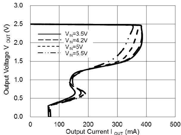
Output Voltage vs. Output Current AP7340-25
