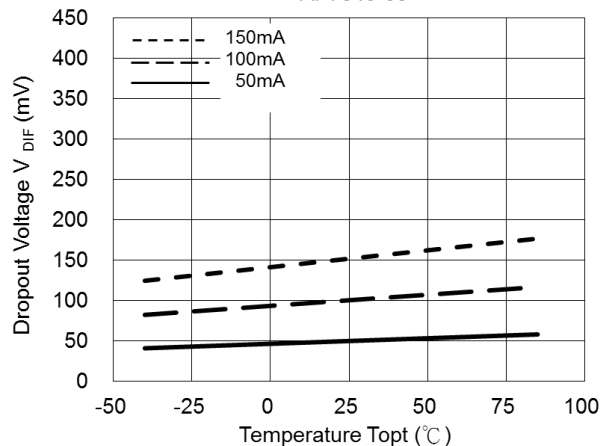
Dropout Voltage vs. Temperature AP7340-33
