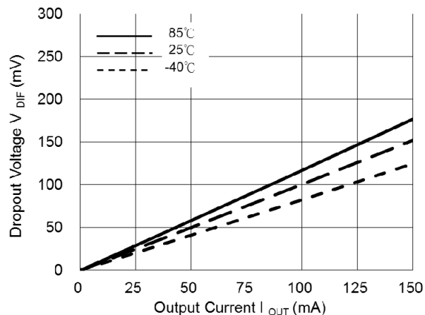
Dropout Voltage vs. Output Current AP7340-33
